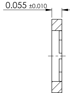
SECTION Y-Y
